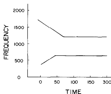
FIG. 14. Schematic diagram of a syllable that will be heard as /ga/ or /ka/, depending on the point in the syllable at which voicing begins. Prior to the onset of voicing, F2 (top curve) is energized by aperiodic noise sources, and F1 is "cut back" (the noise source has little or no energy in this range). Because of the fact that F1 rises over time after syllable onset (as the vocal tract moves from a shape consistent with the consonant into a shape consistent with the vowel), its frequency at the onset of voicing is higher for later values of VOT. Parameters used in constructing this schematic syllable are derived from Kewley-Port's (1982) analysis of the parameters of formants in natural speech, and are similar to those used in many perceptual experiments.
