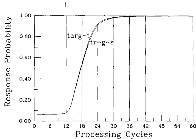
FIG. 10. Time course of growth in the probability of the /t/ response based on activations of phoneme units in Slice 12, during processing of /targ t / and /tr g s/. The vertical lines indicate the peaks on the feature patterns corresponding to the successive phonemes of the presented word.
