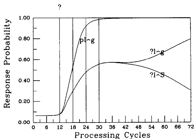
FIG. 6. The time course of the buildup in the strength of the /p/ response based on activations of phoneme units in Slice 12, in processing an ambiguous /b/-/p/ segment in /lˈg/, and the same segment in /lˈS/. The ambiguous segment is indicated by the "?". Also shown is the buildup of response strength for processing an unambiguous /p/ segment in /plˈg/. The vertical line topped with "?" indicates the point in time corresponding to the center of the initial segment in the input stream. Successive vertical lines indicate centers of successive phonemes.
