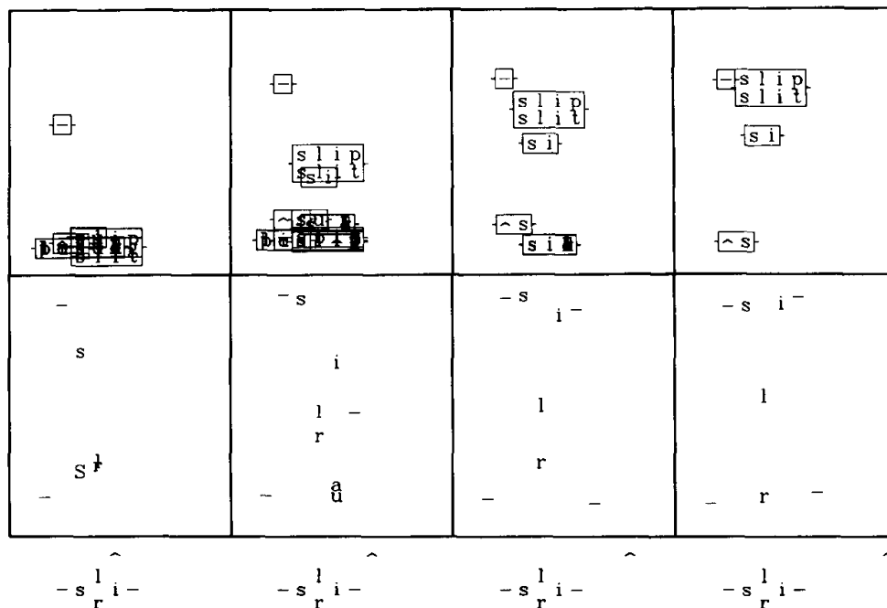
FIG. 12. State of the Trace at several points in processing a segment ambiguous between /l/ and /r/, in the context /sli/. The units for "sleep" (/slip/) and "sleet" (/slit/) are boxed together since they take on identical activation values.
